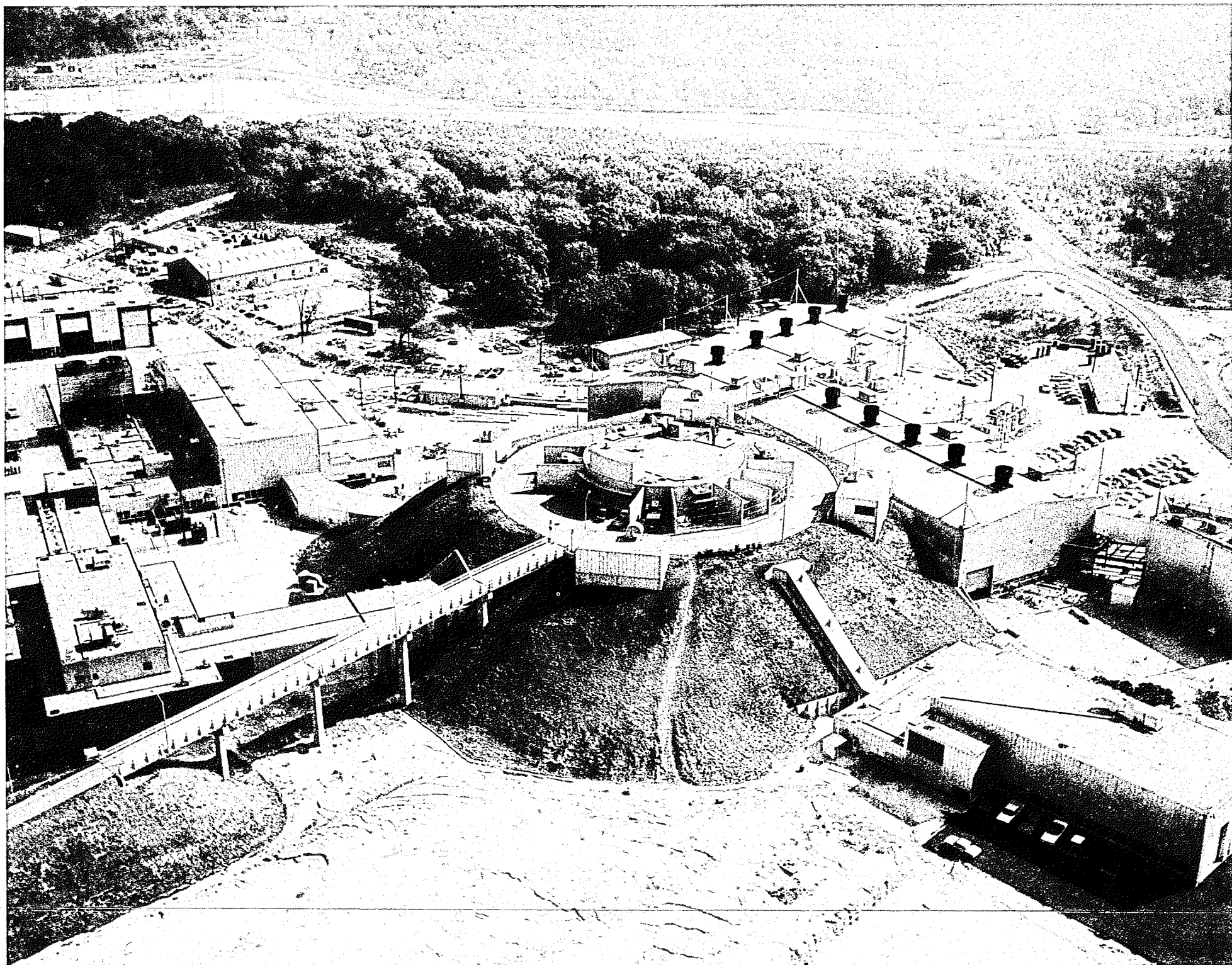
Aerial view of the Zero Gradient Synchrotron (ZGS) at Argonne National Laboratory, taken September 26, 1963. A mound of earth, approximately 50 feet high, covers the doughnut-shaped magnet ring building, which is 212 feet in diameter. Inside this building, within a 200-foot ring of steel magnets weighing a total of 4800 tons, tiny protons--the nuclei of hydrogen atoms--are accelerated to 12.5 billion electron volts. The protons and beams of "secondary" particles are shot into experimental buildings at right. At left, behind the road leading to the top of the mound, are buildings that house the beam injector and control systems of the ZGS. At right foreground is the magnet power supply building.
